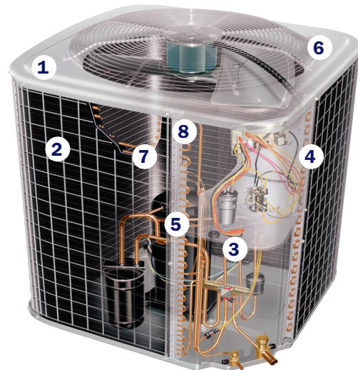
Heat Pump
